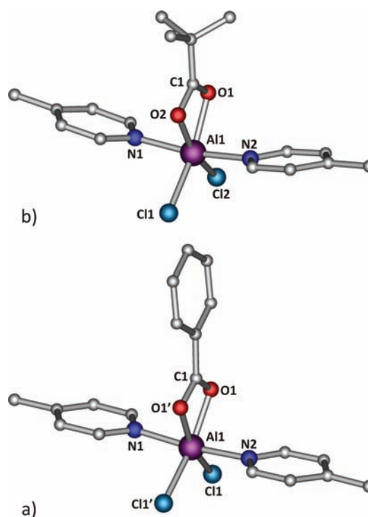
Figure 4. Molecular structures of (a) 3a and (b) 3b ; hydrogen atoms have been omitted for clarity. Selected bond lengths (Å) and angles (deg): (a): Al1-Cl1 , 2.232(1); Al1-Cl1' , 2.232(9); Al1-O1 , 1.975(2); Al1-O1' , 1.975(2); Al1-N1 , 2.057(3); Al1-N2 , 2.065(3); N1-Al1-N2 , 174.1(1); O1-C1-O1' , 115.8(3); O1-Al1-O2 , 66.4(1); (b): Al1-Cl1 , 2.249(1); Al1-Cl2 , 2.214(1); Al1-O1 , 1.986(2); Al1-O2 , 1.977(2); Al1-N1 , 2.043(3); Al1-N2 , 2.046(3); N1-Al1-N2 , 170.2(1); O1-C1-O2 , 115.7(3); O1-Al1-O2 , 65.9(1).
