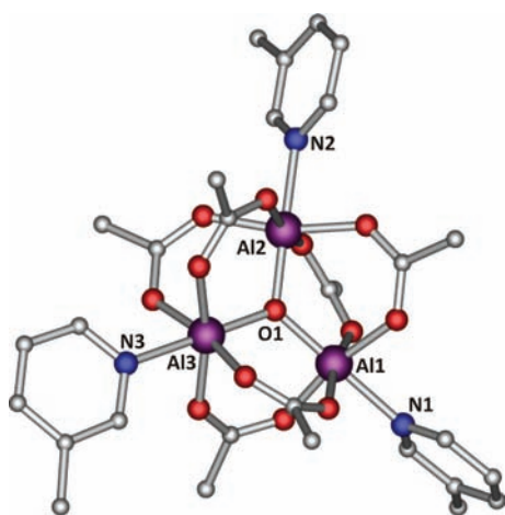
Figure 8. Molecular structure of 4b py-Me ; hydrogen atoms and methyl groups of t Bu have been omitted for clarity. Selected bond lengths (Å) and angles (deg): O1–Al1, 1.819(4); O1–Al2, 1.827(4); O1–Al3, 1.820(4); Al1–N1, 2.096(5); Al2–N2, 2.102(5); Al3–N3, 2.103(5); Al1–O1–Al2, 119.7(2); Al1–O1–Al3, 120.7(2); Al2–O1–Al3, 119.6(2).
